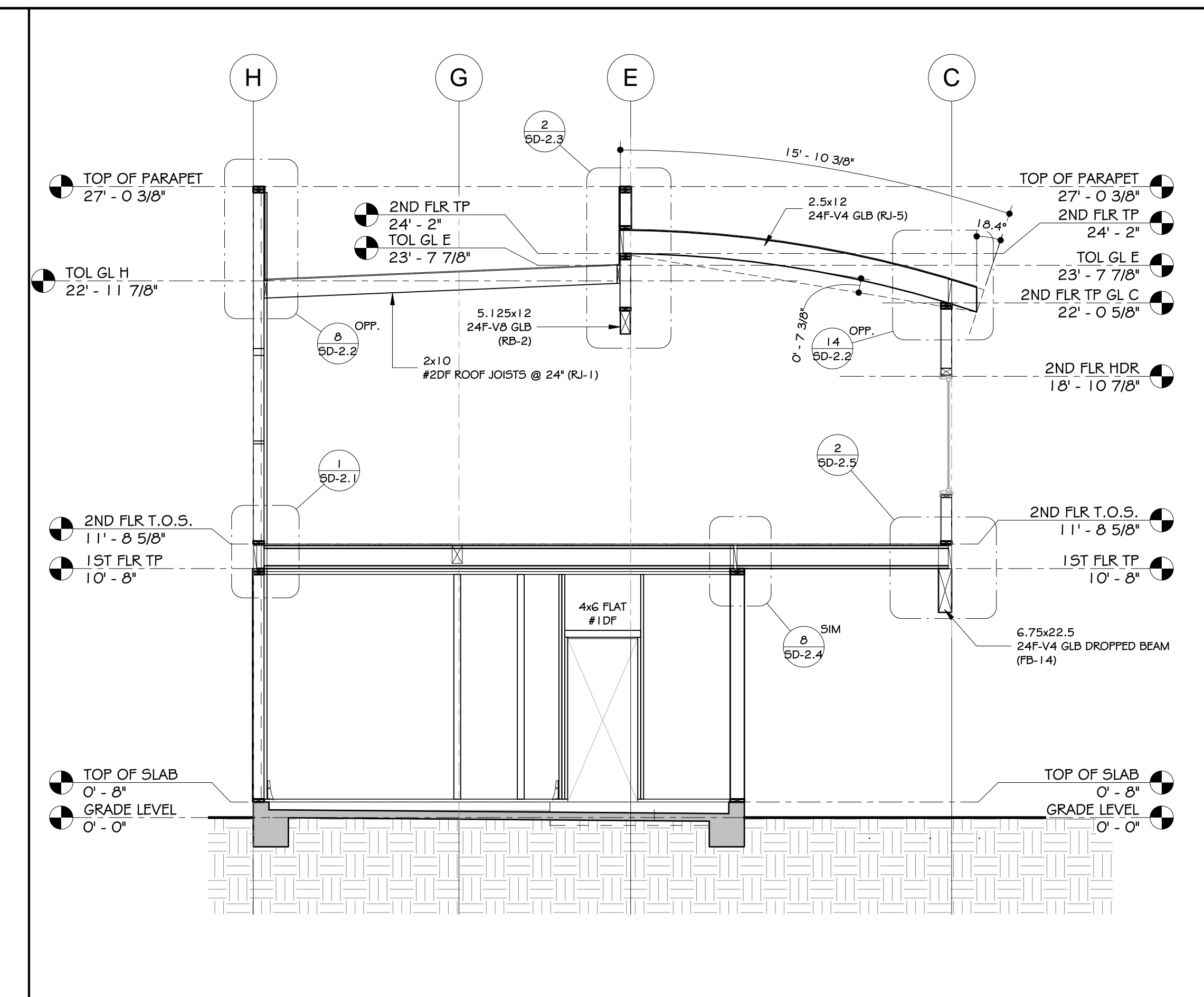
FRAMING ELEVATION GL 1 SCALE: 1/4" = 1'-0"
