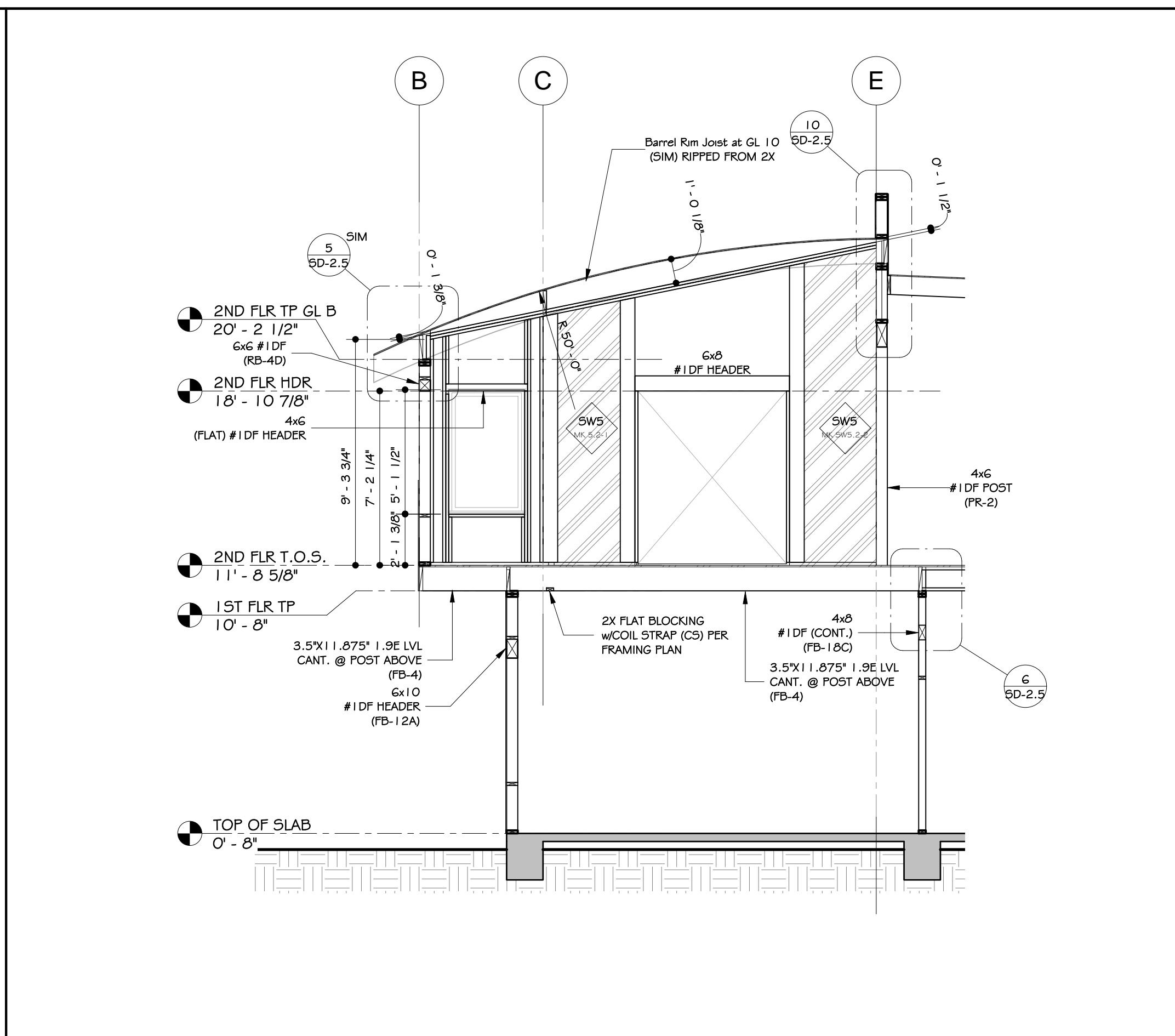
FRAMING ELEVATION AT GL 5 BETWN. GL B AND GL E SCALE: 1/4" = 1'-0"
