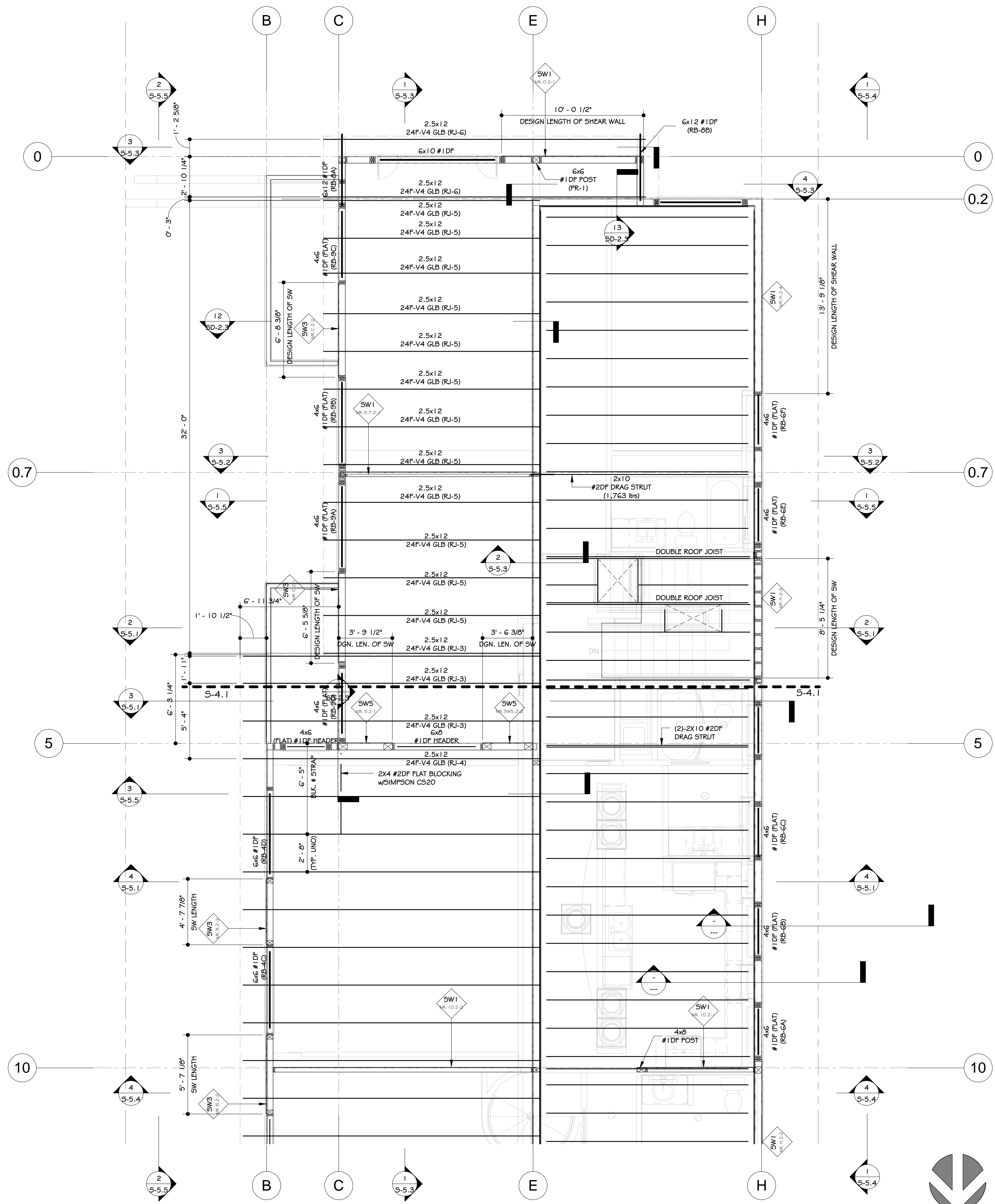
ROOF FRAMING PLAN - SOUTH SCALE: 1/4" = 1'-0"
