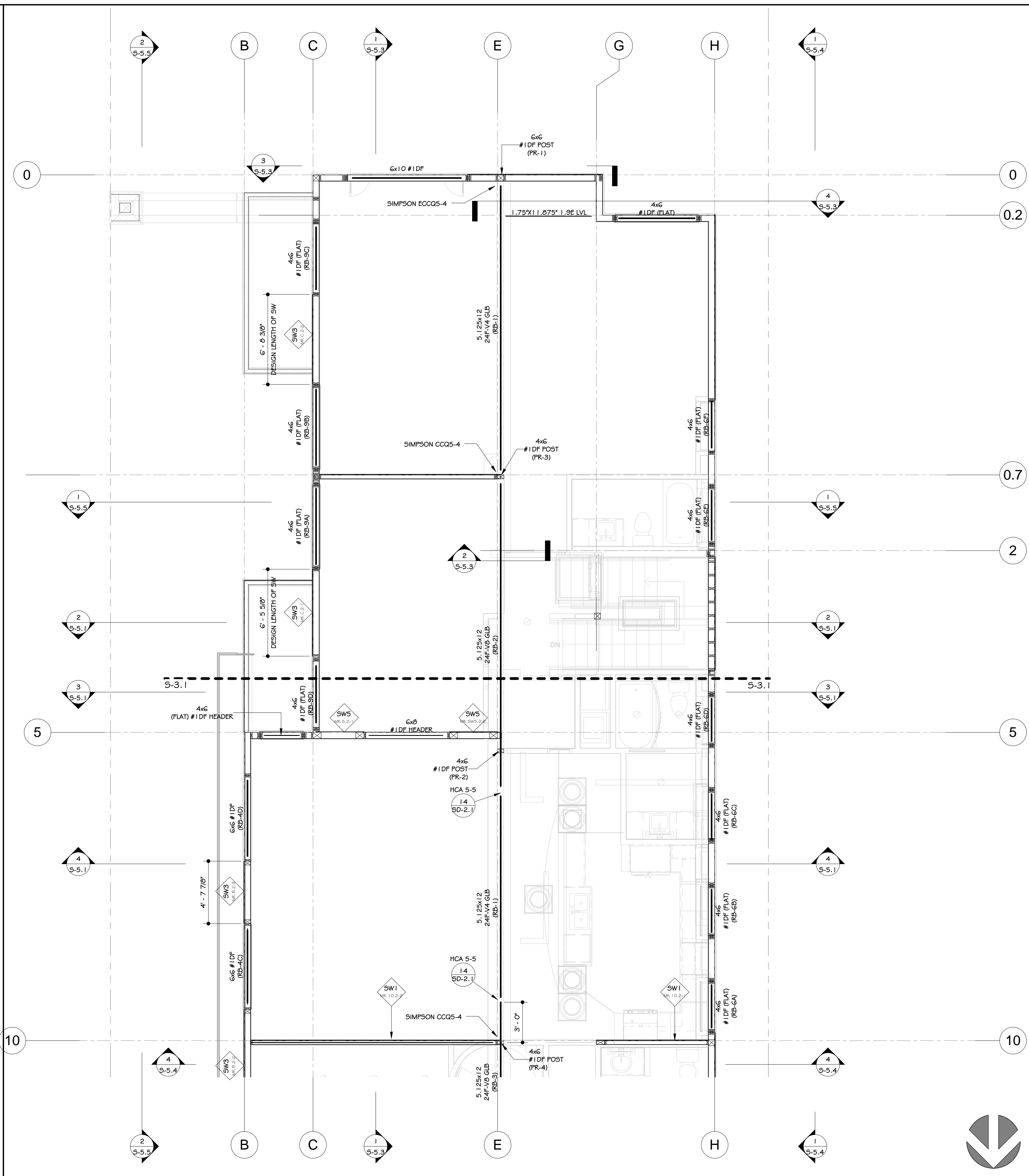
2ND FLOOR CEILING FRAMING PLAN-SOUTH SCALE: 1/4" = 1'-0"
