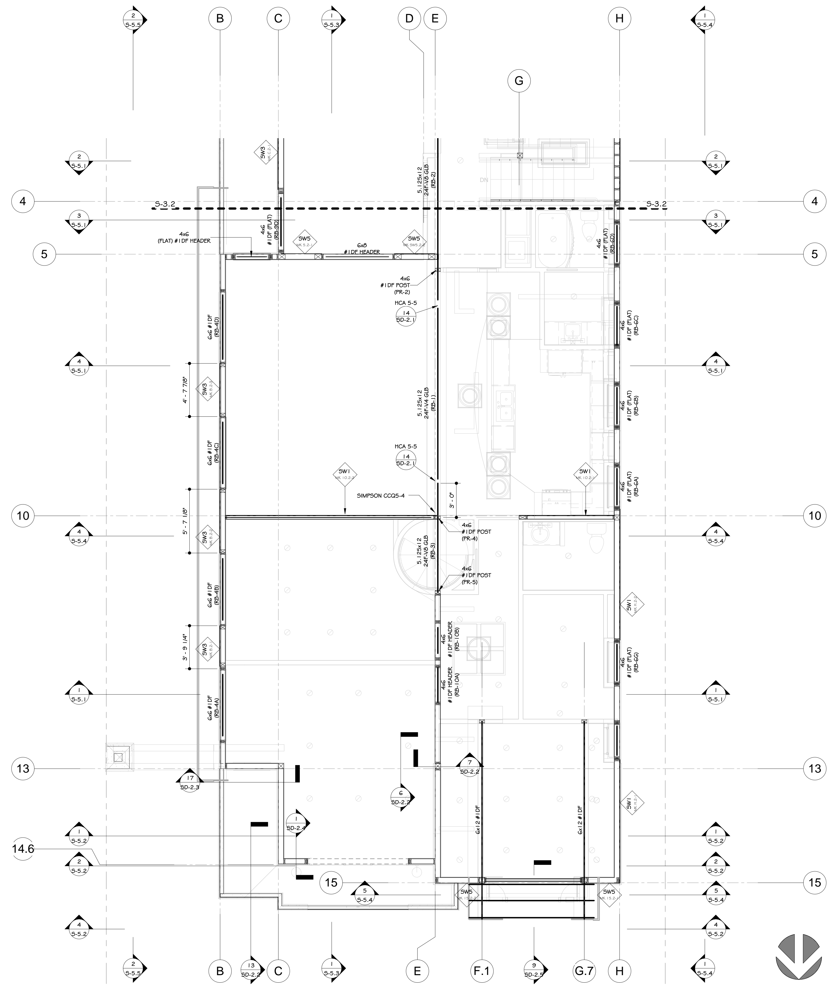
2ND FLOOR CEILING FRAMING PLAN-NORTH SCALE: 1/4" = 1'-0"
