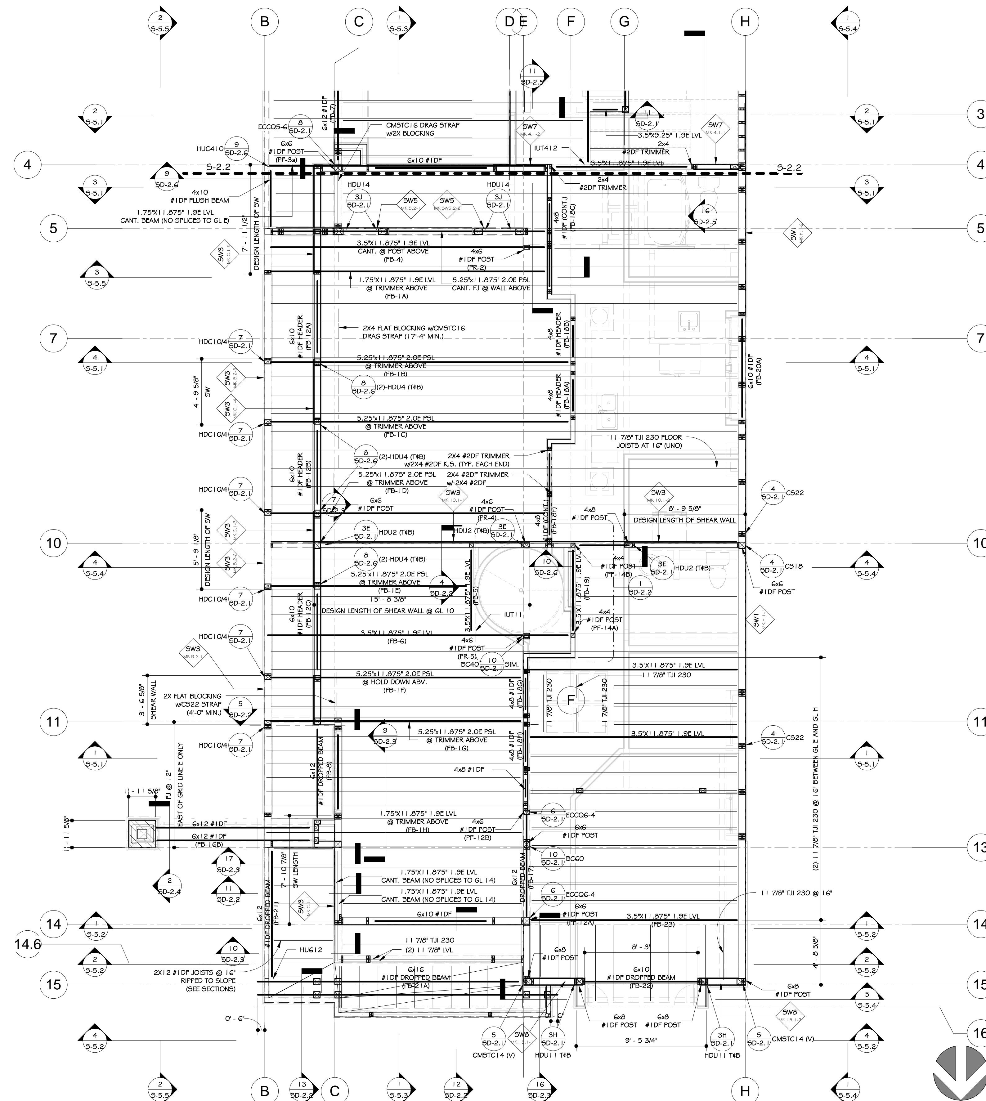
2ND FLOOR FRAMING PLAN-NORTH SCALE: 1/4" = 1'-0"
