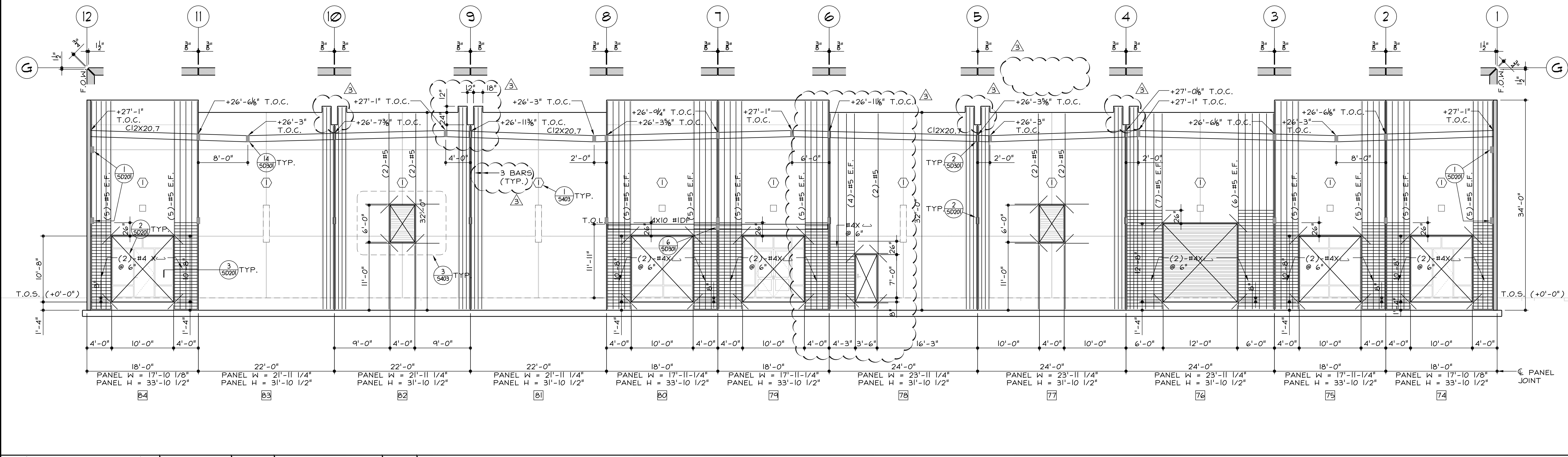
PANEL ELEVATION GRID LINE G - BUILDING B
