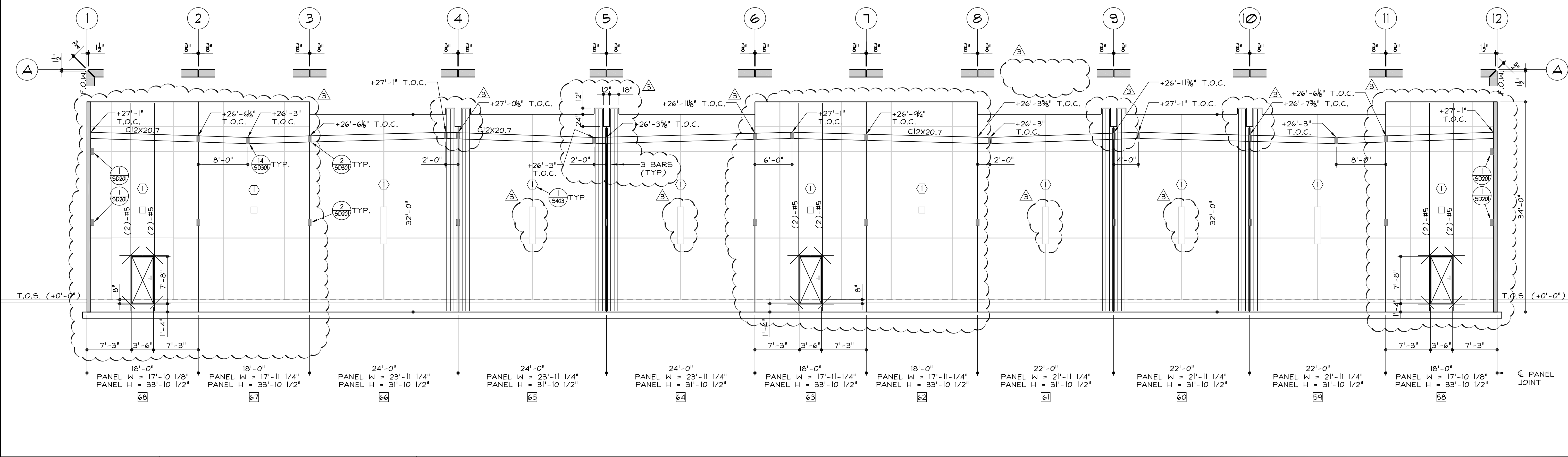
PANEL ELEVATION GRID LINE A - BUILDING B
